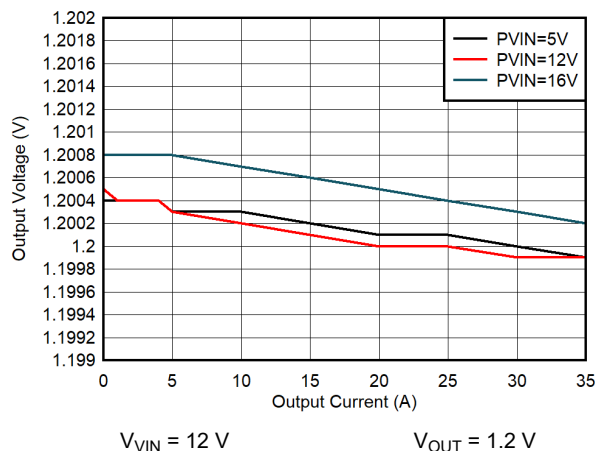
图 9-2. Load Regulation
