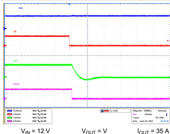
图 9-6. Shutdown from CNTL
