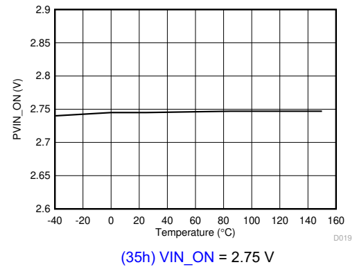
图 7-10. Turn-On Voltage vs Junction Temperature
