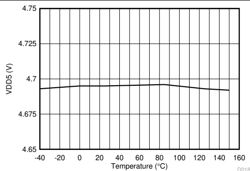
图 6-12. VDD5 Voltage vs Junction Temperature
