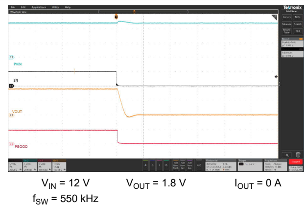
图 8-22. Shutdown from CNTL
