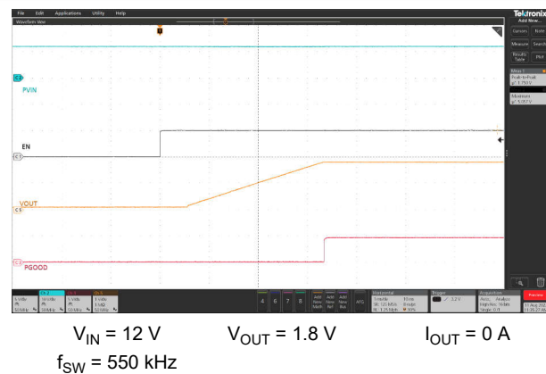
图 8-21. Start-Up from EN/UVLO
