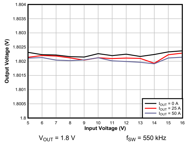
图 8-20. Line Regulation
