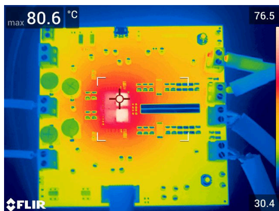
图 8-29. Thermal Image at 25°C Ambient, 12 V IN , Dual 1.0 V OUT , 25 A, 550 kHz
