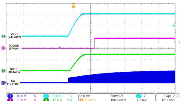
I_{OUT} = 15\text{ A} FCCM
