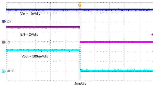
图 8-14. Shutdown Through EN, I_{OUT} = 3A
