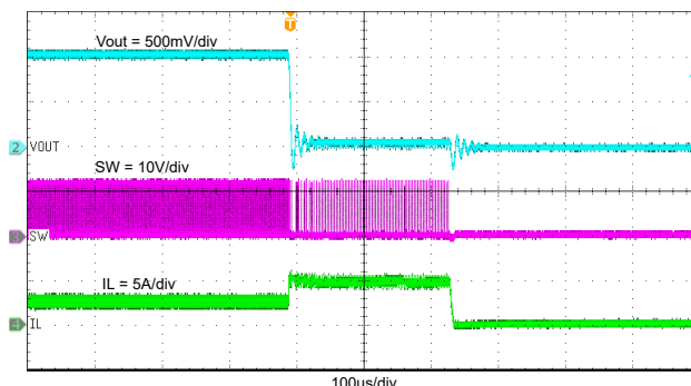
图 8-17. TPSM863252 Normal Operation to Output Hard Short
