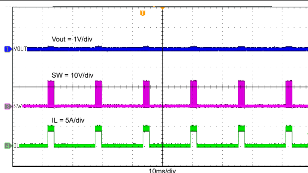
图 8-19. Output Hard Short Hiccup
