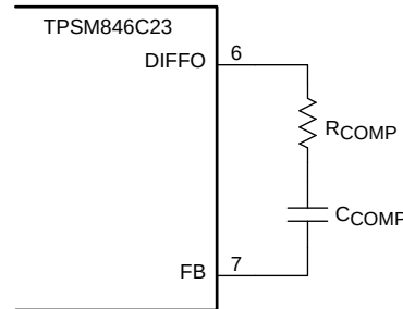
图 14. Compensation Components
