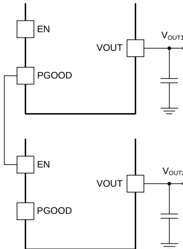
图 22. Sequencing Schematic
