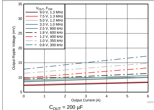
图 3. Ripple Voltage vs Output Current
