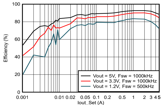
TPSM84538 效率, V_{IN} = 12V . PFM
