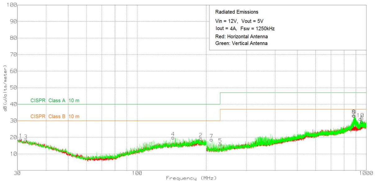
图 31. Radiated Emissions 12-V Input, 5-V Output, 4-A Load (EN55011 Class B)
