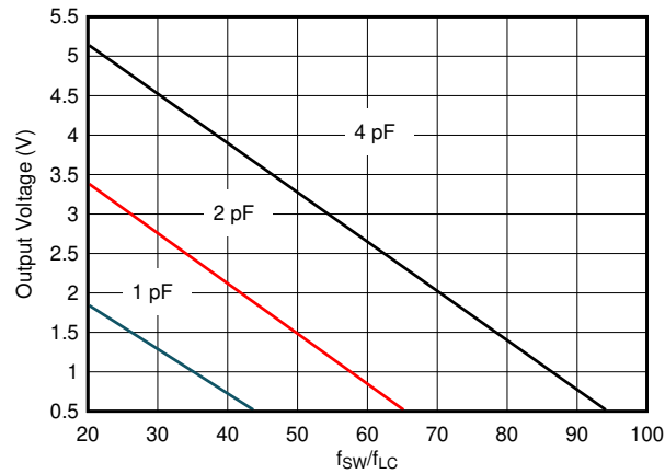
图 7-3. Recommended Ramp Settings
