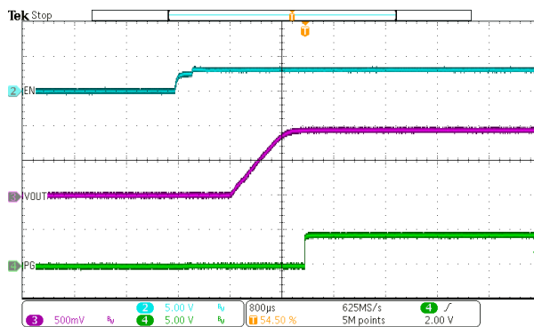
V_{IN} = 12V I_{OUT} = 3A 图 7-11. EN Start-Up – With Load
