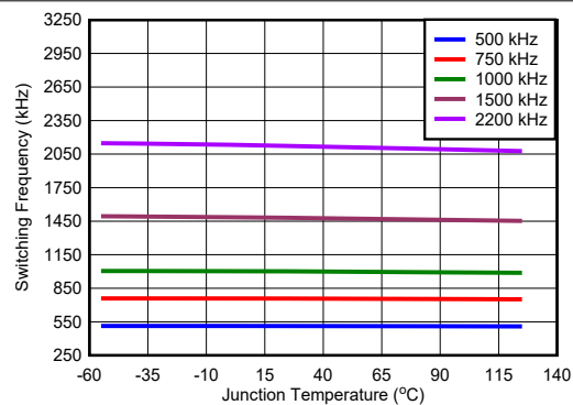
图 5-12. Switching Frequency
