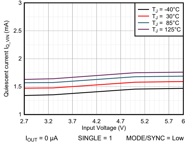
图 6-1. Operating Supply Current (Power-Save Mode)
