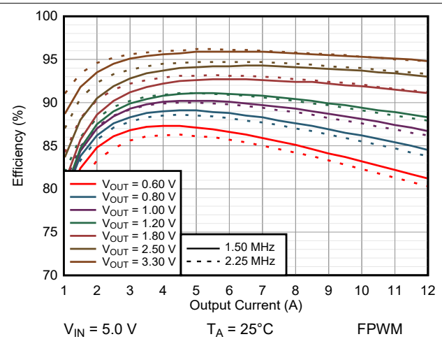
图 7-15. Efficiency Comparison TPSM8287A12BAS vs TPSM8287A12BBS
