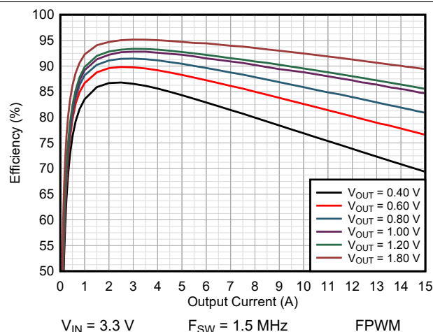
图 9-16. Efficiency TPSM8287A15BAH
