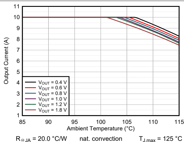
图 9-40. Safe Operating Area TPSM8287A10BAH V_{IN} = 3.3\text{ V}
