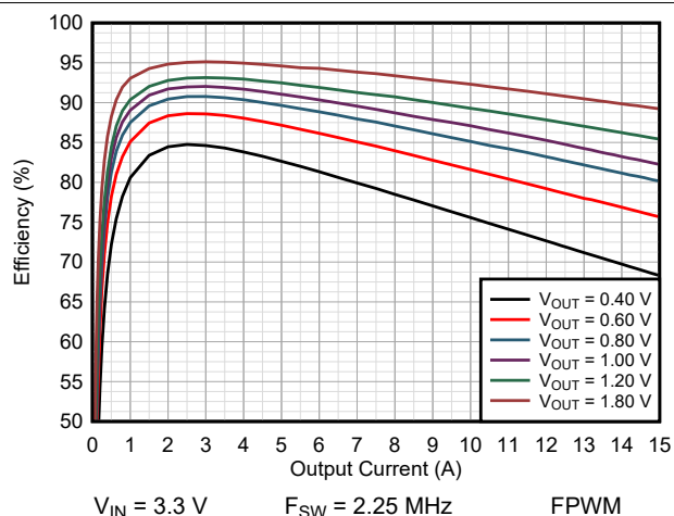
图 9-17. Efficiency TPSM8287A15BBH
