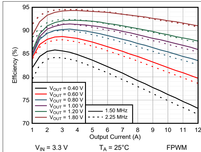
图 7-14. Efficiency Comparison TPSM8287A12BAS vs TPSM8287A12BBS
