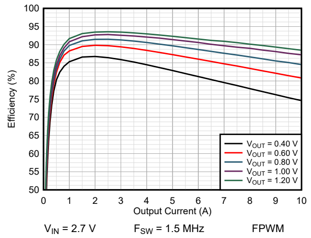
图 9-3. Efficiency TPSM8287A10BAH
