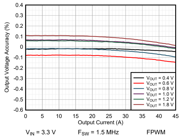
图 9-54. Load Regulation
