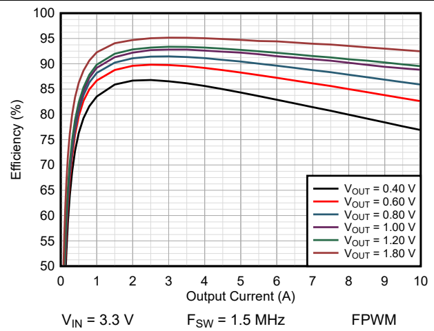
图 9-5. Efficiency TPSM8287A10BAH
