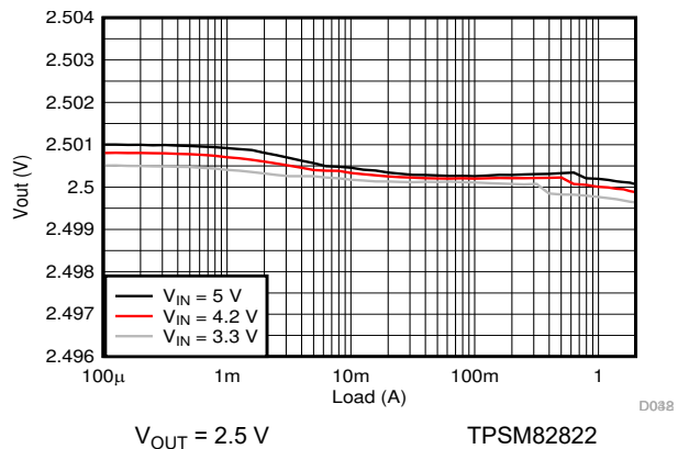
图 9-69. Load Regulation
