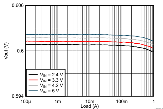
图 9-42. Load Regulation
