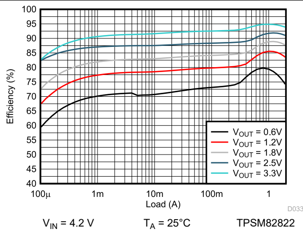
图 9-55. Efficiency
