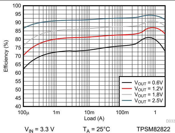
图 9-57. Efficiency
