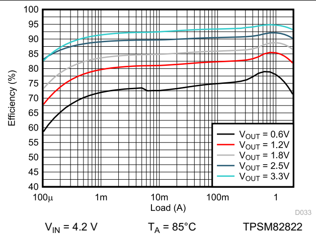
图 9-56. Efficiency
