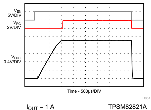
图 9-51. Start-up / Shutdown with Resistive Load
