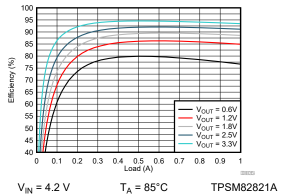
图 9-32. Efficiency
