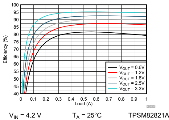
图 9-31. Efficiency
