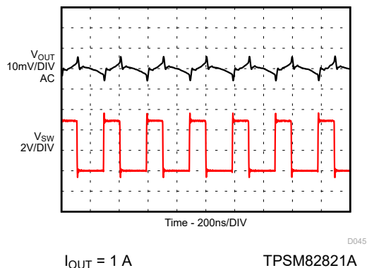
图 9-47. Output Ripple in PWM Mode
