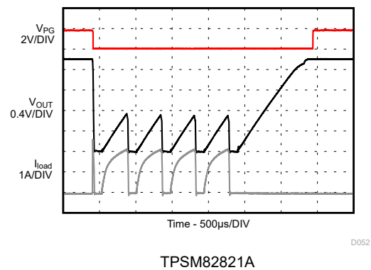
图 9-52. Short Circuit, HICCUP Protection Entry / Exit
