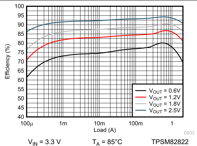
图 9-58. Efficiency
