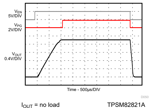
图 9-50. Start-up / Shutdown without Load
