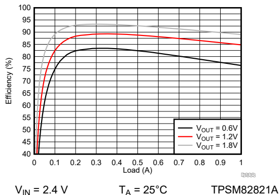
图 9-35. Efficiency
