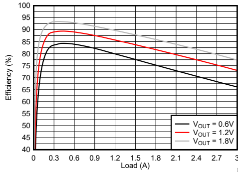
图 9-143. Efficiency
