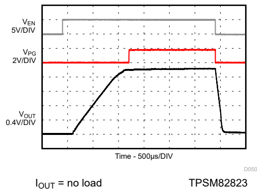
图 9-133. Start-up / Shutdown without Load
