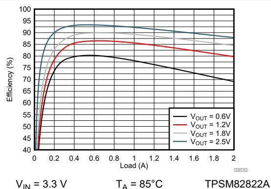
图 9-91. Efficiency
