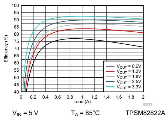
图 9-87. Efficiency
