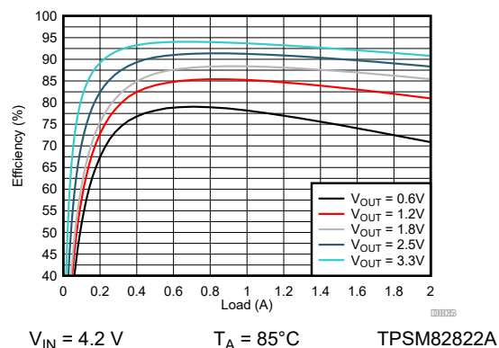
图 9-89. Efficiency
