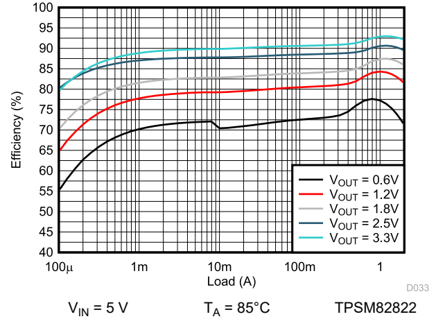
图 9-54. Efficiency
