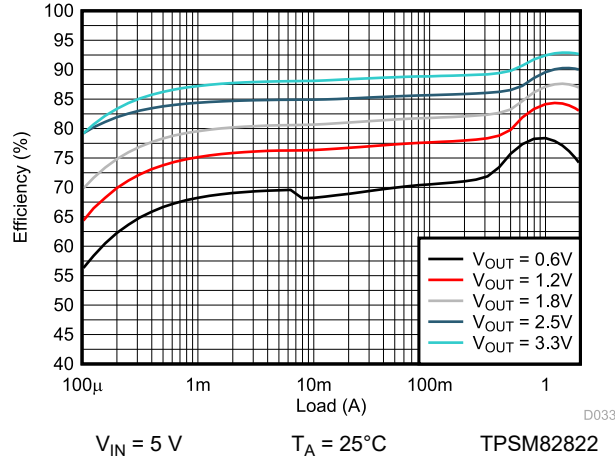
图 9-53. Efficiency
