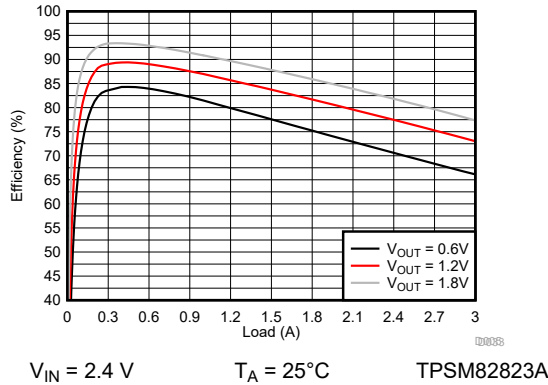
图 9-143. Efficiency
