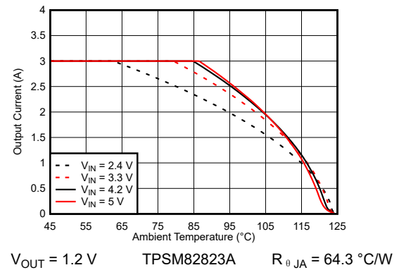
图 9-146. Safe Operating Area
