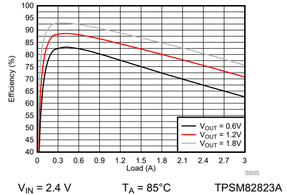
图 9-144. Efficiency
