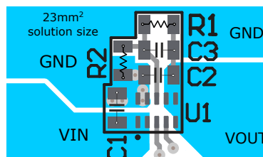
图 11-2. TPSM8282x/TPSM8282xA PCB Layout for the Adjustable Devices (BOM from Table 9-1 with 1 x 22-μF for C2)
