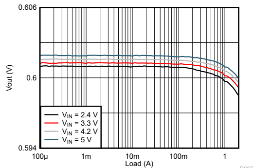
图 9-99. Load Regulation
