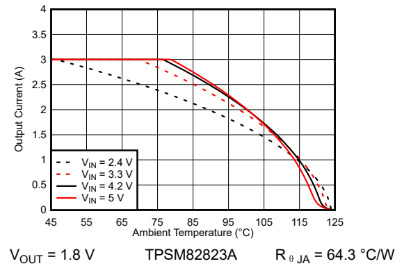
图 9-147. Safe Operating Area
