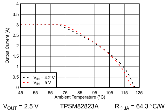
图 9-148. Safe Operating Area
