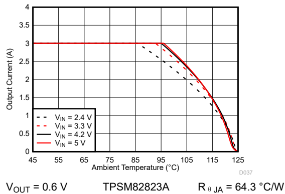
图 9-145. Safe Operating Area
