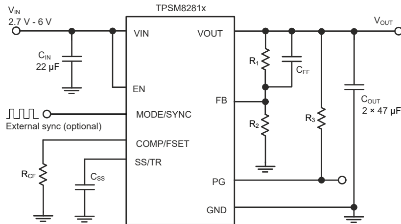
图 8-35. Frequency Synchronization
