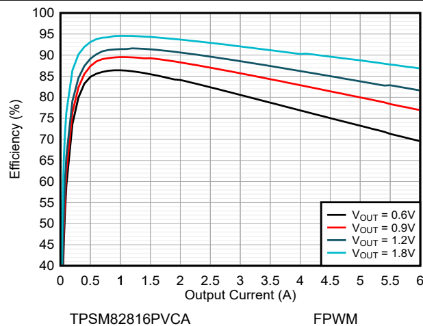
图 8-12. Efficiency V_{IN} = 2.7\text{ V} and T_A = 85^\circ\text{C}
