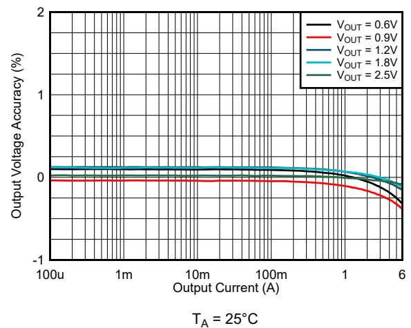
图 8-17. Load Regulation V_{IN} = 3.3\text{ V} (FPWM)
