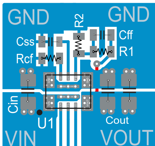
图 9-39. Example Layout SIL Package
