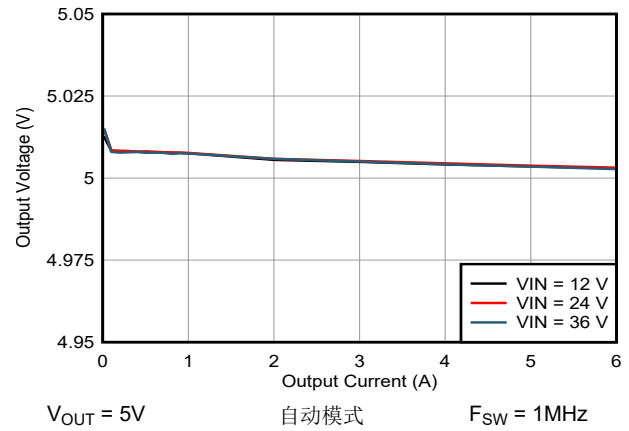
图 9-5. V_{OUT} = 5V 时的负载调节
