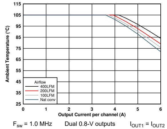
图 6-11. Safe Operating Area ( V_{OUT} = 0.8\text{ V} )
