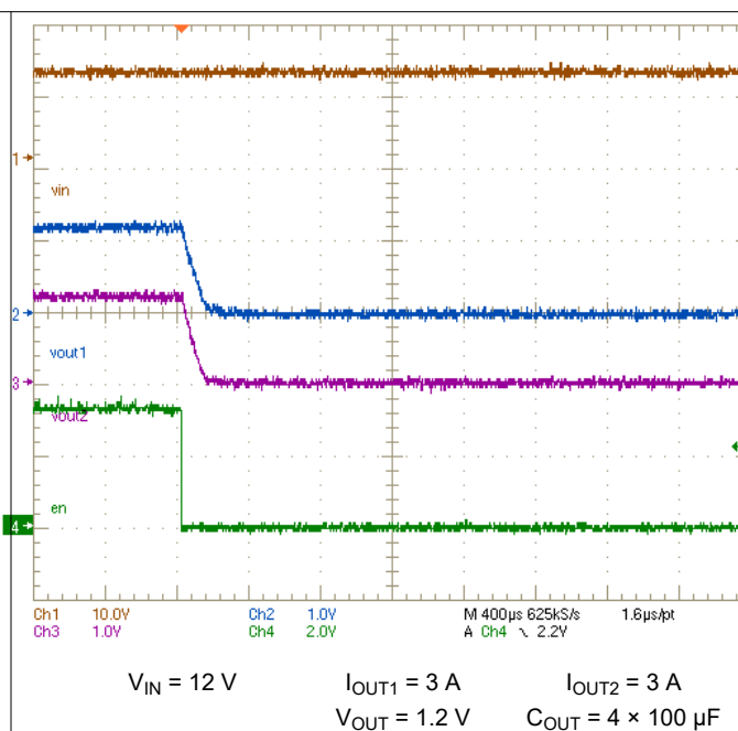
图 8-3. Enable Turn-Off with Load
