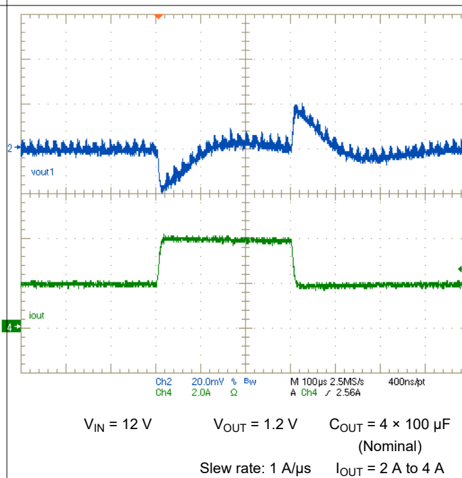
图 8-5. Transient Response V_{OUT1}
