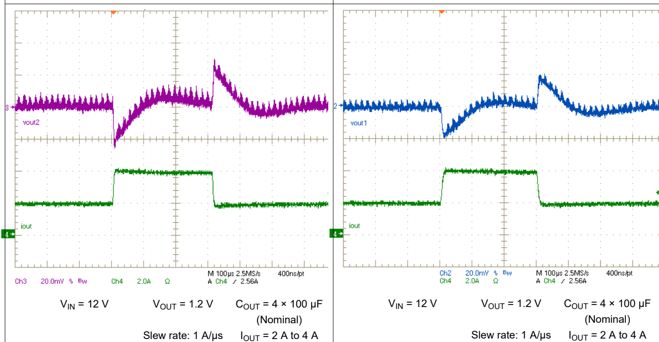
图 8-4. Transient Response V_{OUT2}
