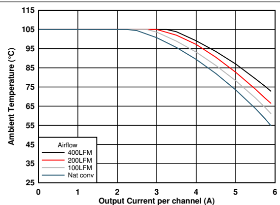
图 6-4. Safe Operating Area ( V_{OUT} = 1.2\text{ V} )
