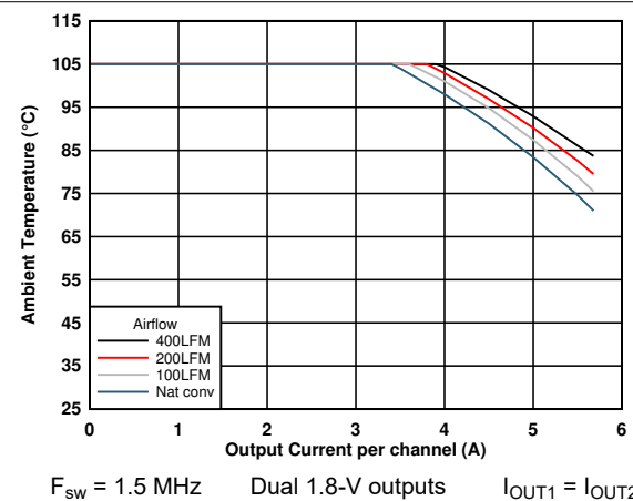
图 6-13. Safe Operating Area ( V_{OUT} = 1.8\text{ V} )
