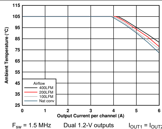
图 6-12. Safe Operating Area ( V_{OUT} = 1.2\text{ V} )
