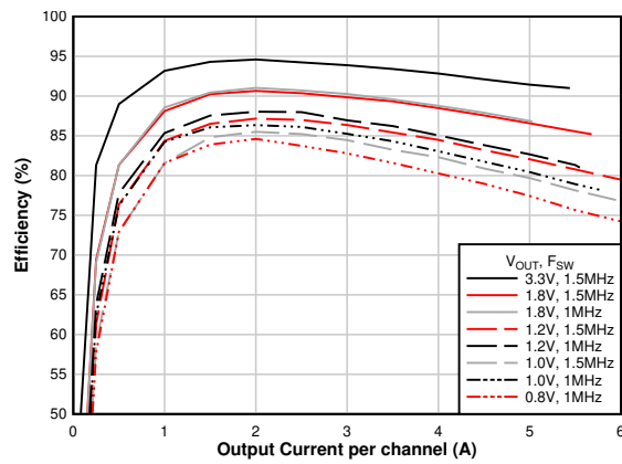
图 6-8. Efficiency vs Output Current
