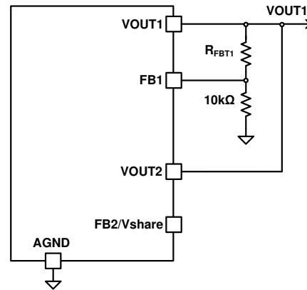
图 7-2. Single Device, Current Sharing
