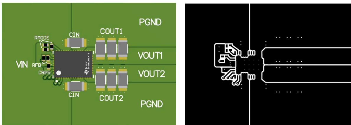
图 10-1. Typical Dual-Output Layout
