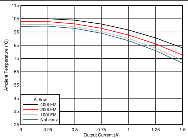
图 7-22. Safe Operating Area ( V_{OUT} = 5.0\text{ V} )
