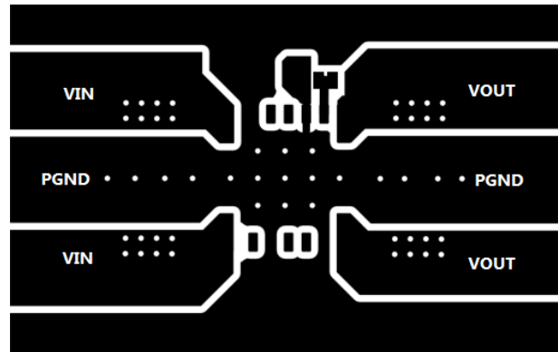
图 11-2. Typical Top-Layer
