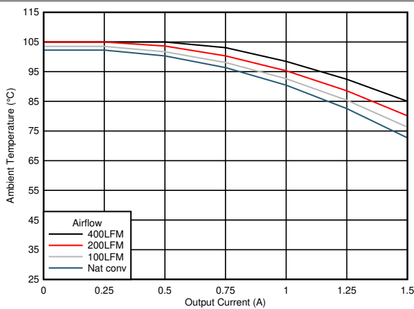
图 7-23. Safe Operating Area ( V_{OUT} = 12\text{ V} )
