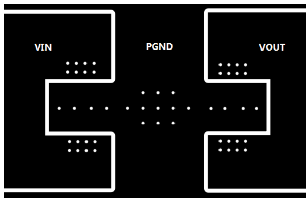
图 11-3. Typical Mid-Layer
