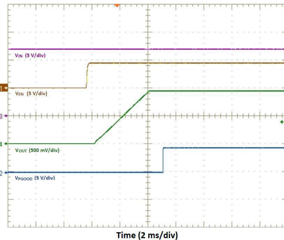
图 8-3. Start-Up Waveforms
