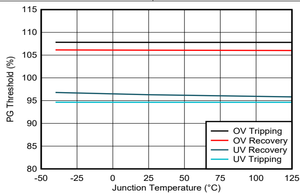
图 8-5. 电源正常 (PG) 阈值
