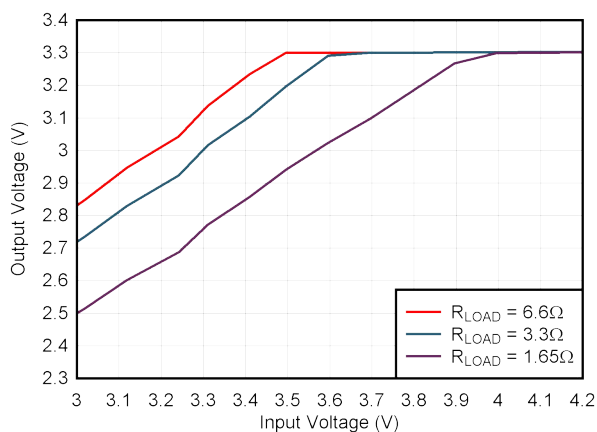
图 8-16. 压降, 12VIN, 3.3VOUT, 2.2MHz (FPWM)
