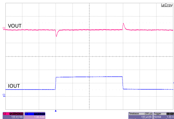
图 8-15. 负载瞬态, 12VIN, 3.3VOUT, 2.2MHz (FPWM), 0.5A 至 1.5A, 1A/μs, COUT = 两个 22 μF
