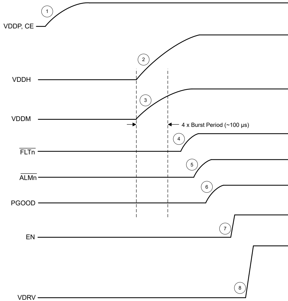
图 8-11. TPSI310x-Q1 典型启动 ( CE = VDDP , FLTn_CMP = 0 , ALMn_CMP = 0 )
