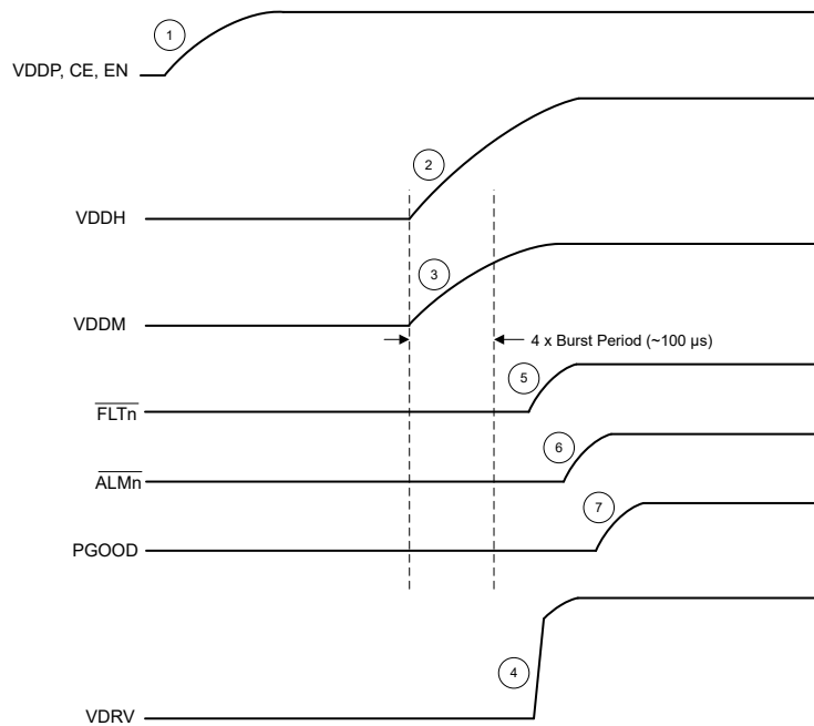
图 8-12. TPSI310x-Q1 典型启动 ( \text{CE} = \text{EN} = \text{VDDP} , \overline{\text{FLTn\_CMP}} = 0 , \overline{\text{ALMn\_CMP}} = 0 )
