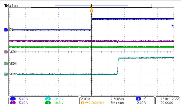
图 9-7. Three-Wire Mode, f_{EN} = 10\text{ kHz} , TPSI3052
