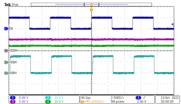
图 9-5. t_{LH\_VDRV} , Three-Wire Mode, TPSI3052
