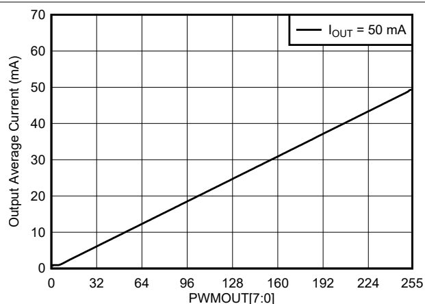
图 5-6. Average Current vs PWMOUT[7:0]
