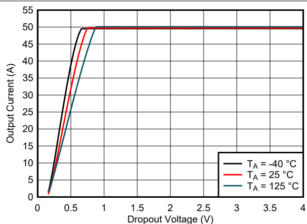
图 5-4. Output Current vs Dropout Voltage
