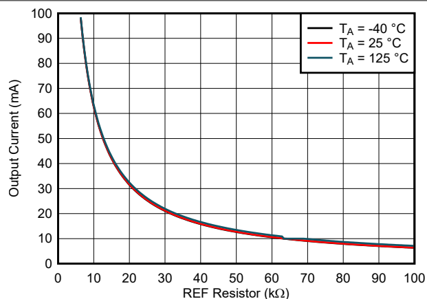
图 5-2. Output Current vs REF Resistor
