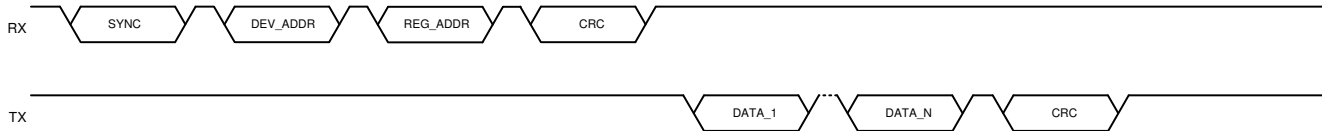
图 6-19. Multiple Data Bytes Read in Burst Mode
