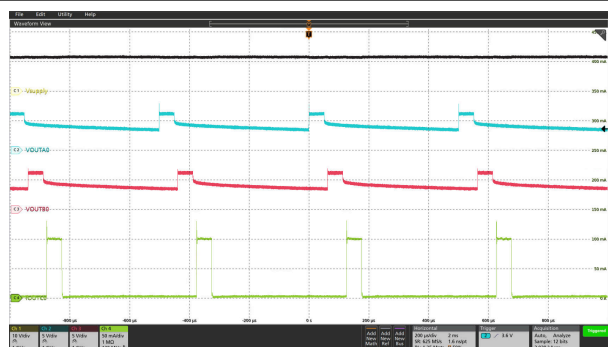
图 5-13. PWM Dimming at 2000Hz
