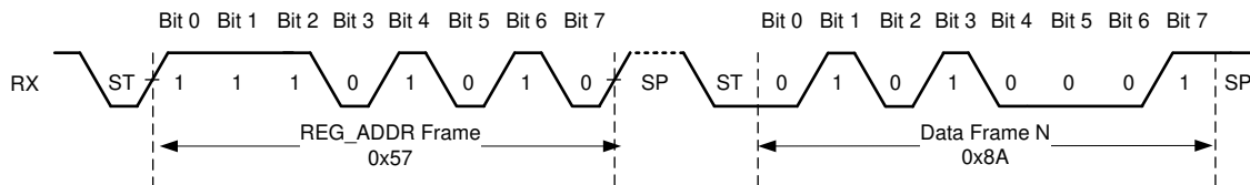
图 6-16. Address and Data Bytes
