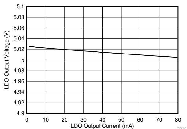
图 6-10. LDO Output Load Regulation
