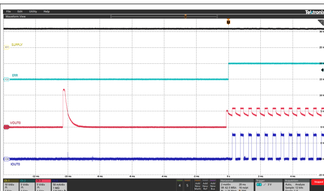
图 6-26. LED Open-Circuit Recovery In FS Mode
