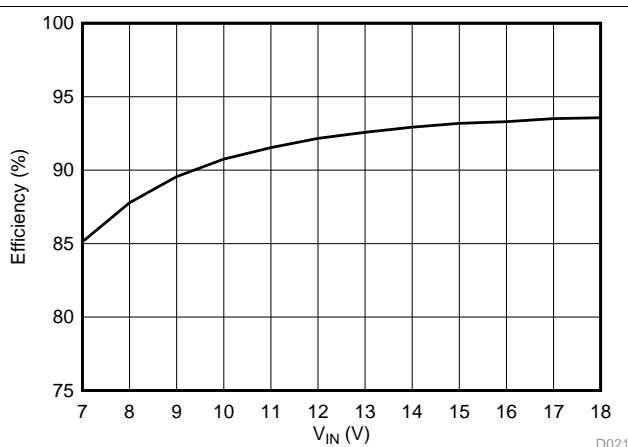
Figure 33. Efficiency vs Input Voltage
