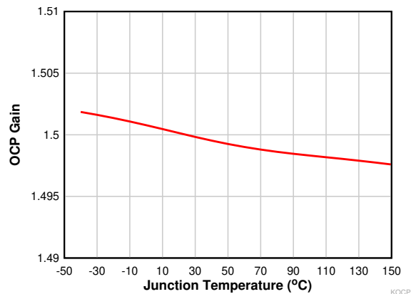
图 6-21. Over Current Protection Gain vs Junction Temperature
