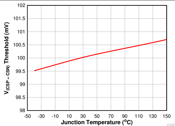
图 6-20. V_{(CSP - VCSN)} Voltage vs Junction Temperature
