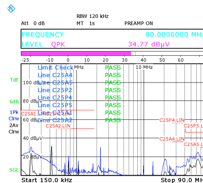
图 8-30. CV Conducted EMI Scan, f_{SW} = 200\text{ kHz}
