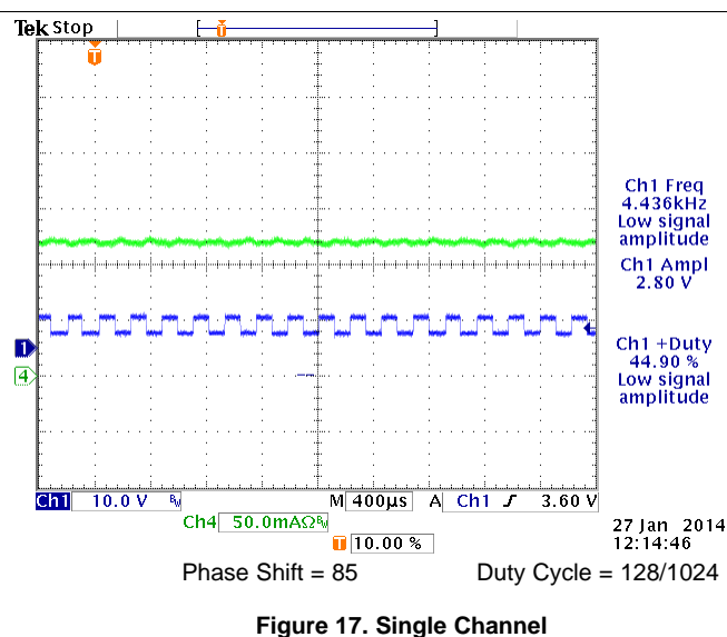
Figure 17. Single Channel
