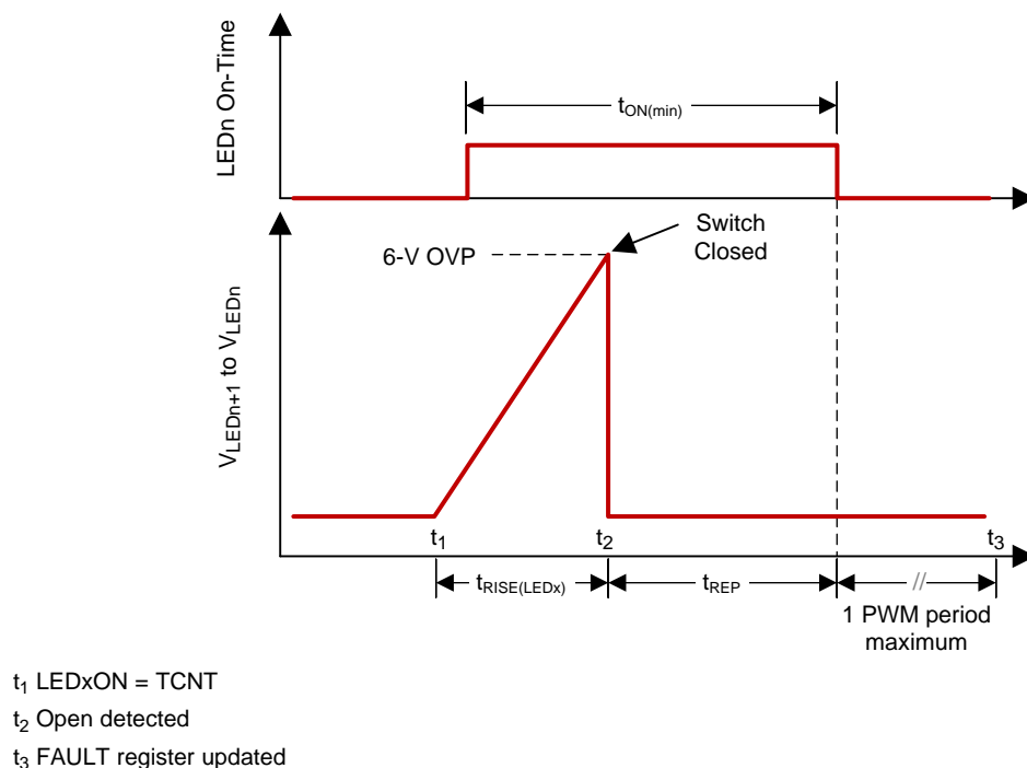
Figure 19. LED Open Fault Detect Timing
