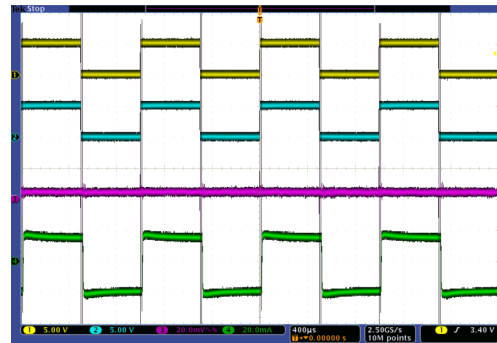
CH1: V_{(PWM3)} CH2: V_{(PWM4)} CH3: V_{(REF)} CH4: I_{(IOUT8)} Duty cycle = 50% V_{(SUPPLY)} , V_{(EN)} = 14 V
