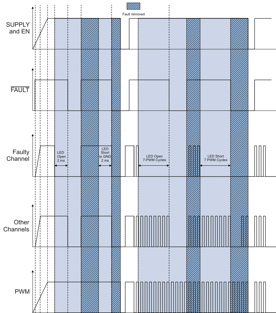
图 32. TPS92638-Q1 Device Fault-Handling Behavior, FAULT Bus Floating
