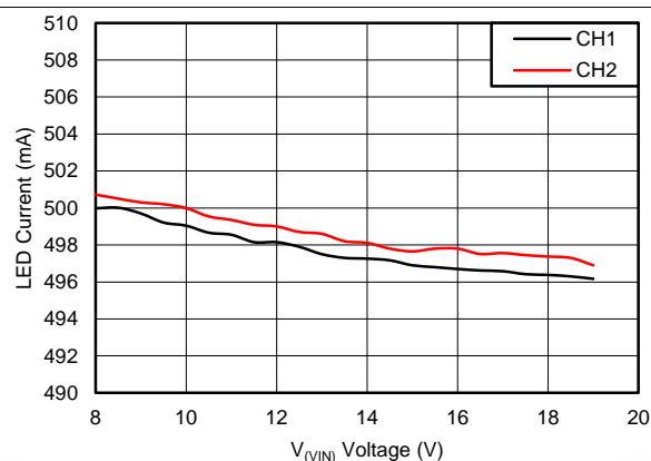
Figure 3. Line Regulation
