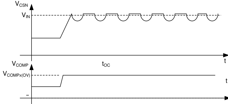
图 7-10. Open Circuit Condition with Output Voltage Oscillation
