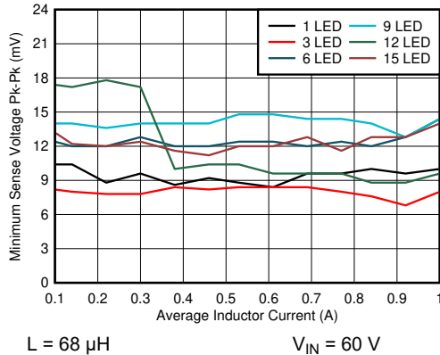
图 6-5. Minimum Ripple Voltage vs Average Inductor Current
