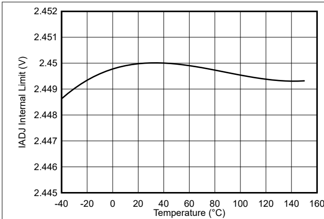
图 6-13. IADJ Internal Limit vs Temperature
