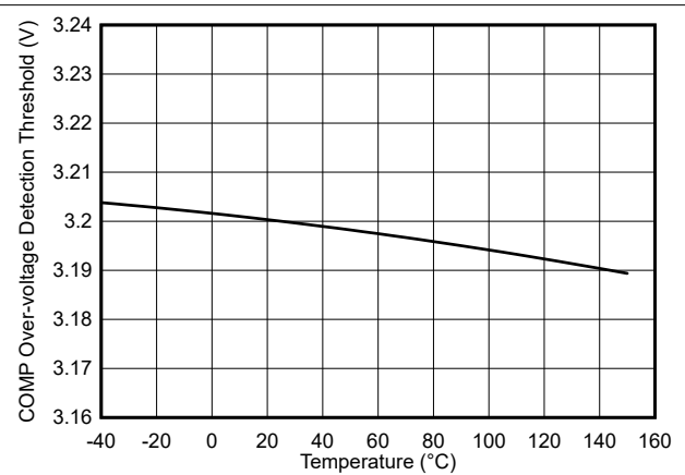
图 6-18. COMP Overvoltage Detection Threshold vs Temperature
