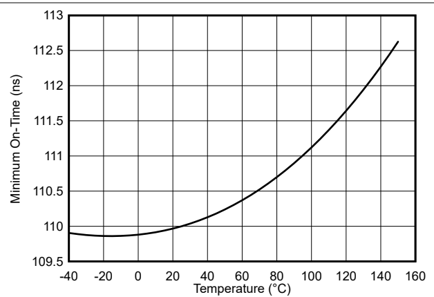
图 6-14. Minimum On-time vs Temperature
