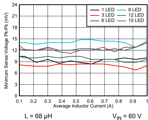
图 6-4. Minimum Ripple Voltage vs Average Inductor Current
