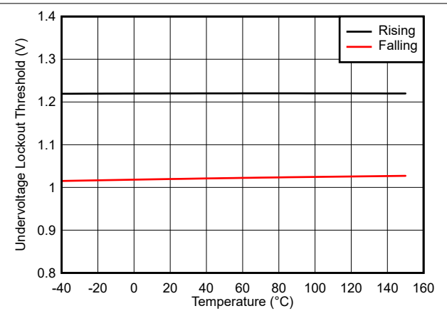
图 6-16. UDIM Undervoltage Lockout Threshold vs Temperature
