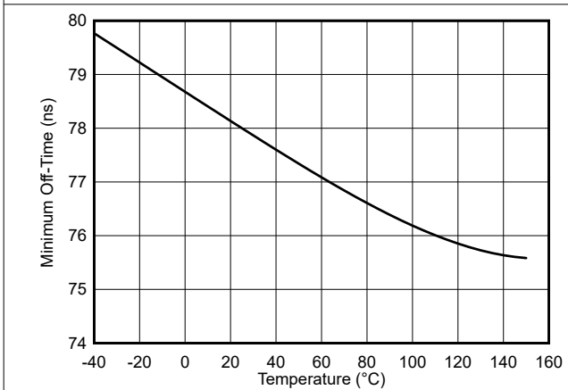
图 6-15. Minimum Off-time vs Temperature
