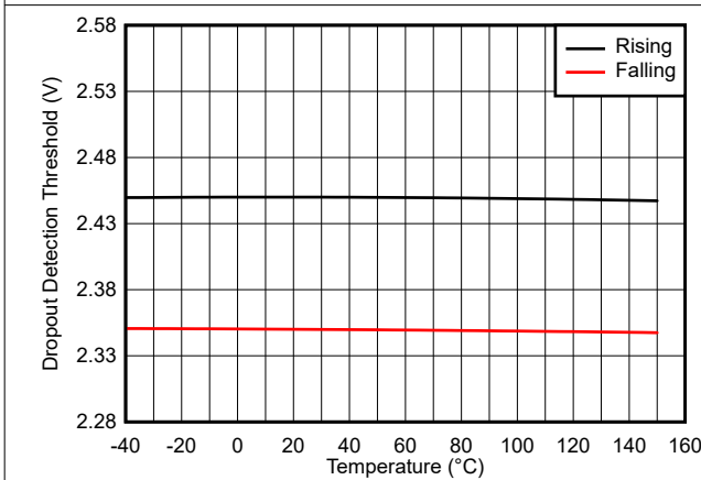
图 6-17. UDIM Dropout Detection Threshold vs Temperature
