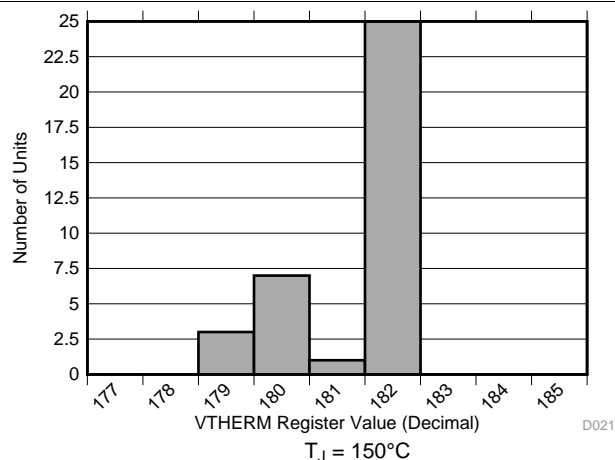
Figure 14. VTherm Performance
