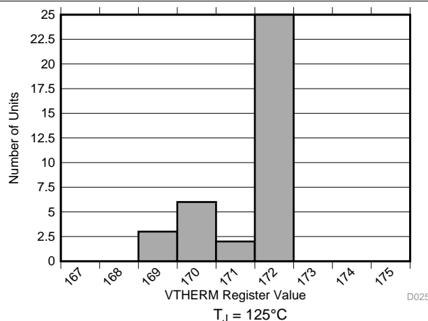
Figure 13. VTherm Performance
