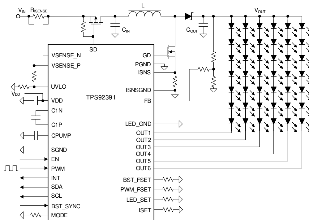
图 8-1. Full Feature Application for Display Backlight
