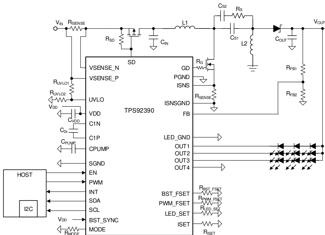
图 8-7. SEPIC 模式 with Three LEDs in Series
