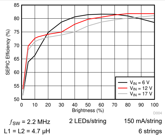
图 6-5. SEPIC Efficiency
