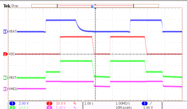
图 9-4. 15V AC/DC Supply with Battery Backup Handoff
