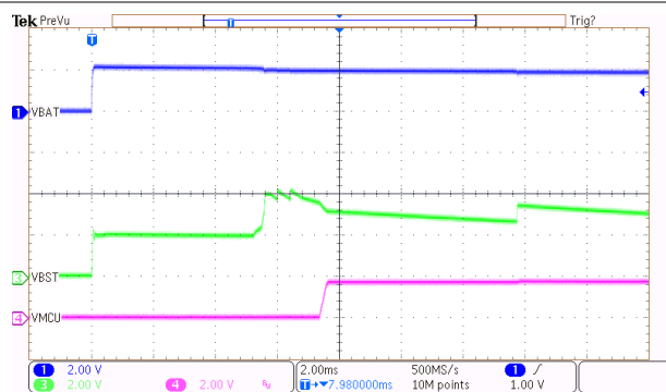
图 9-2. Power-up Waveforms
