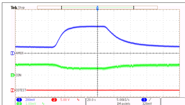
图 9-8. Carbon Monoxide Amplifier Waveforms with Calibration Gas
