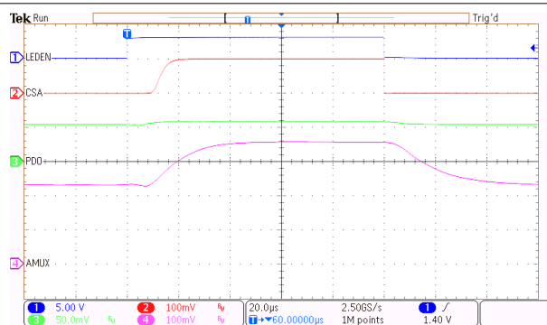
图 9-7. LED Driver and Photo Amplifier Waveforms with 128 Averages
