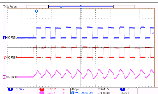
图 9-9. 3-Terminal Horn Driver Waveforms
