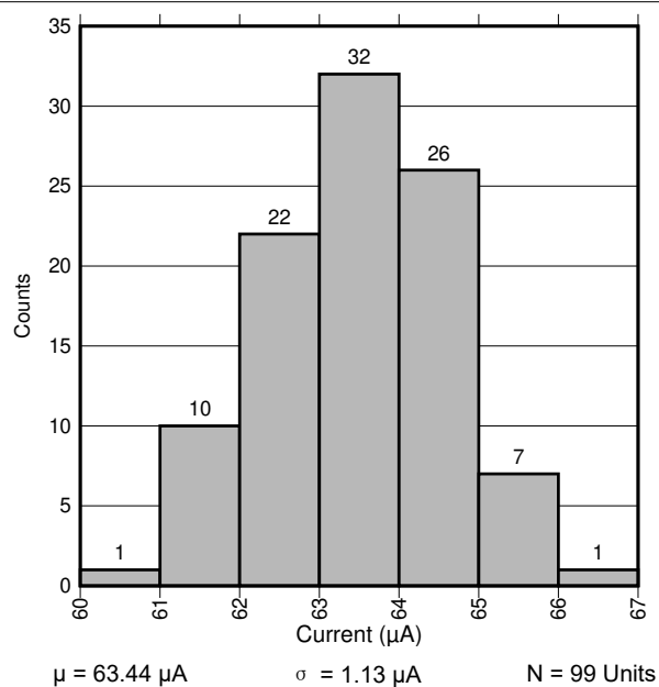
图 7-2. Bias Block Current
