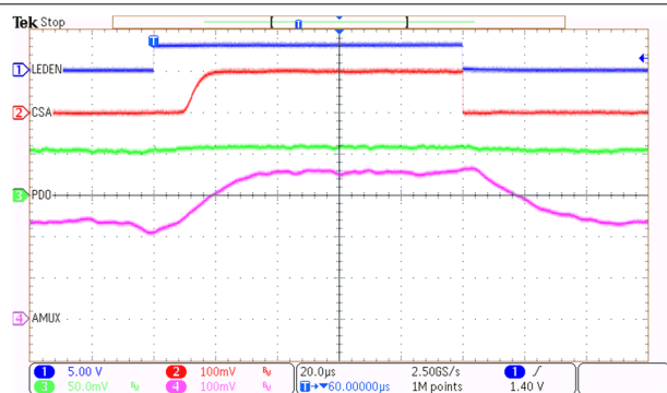
图 9-6. LED Driver and Photo Amplifier Waveforms
