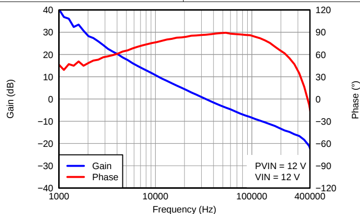
图 5. V_{OUT}=1.2V , I_{OUT}=3A , C_{OUT1}=47\mu F 陶瓷电容器, C_{OUT2}=330\mu F POSCAP, f_{SW}=480kHz
