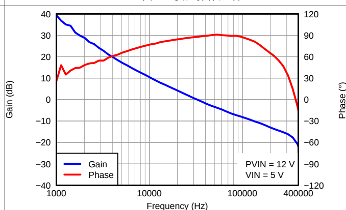
图 16. V_{OUT}=1.2V , I_{OUT}=3A , C_{OUT1}=47\mu F 陶瓷电容器, C_{OUT2}=330\mu F POSCAP, f_{SW}=480kHz
