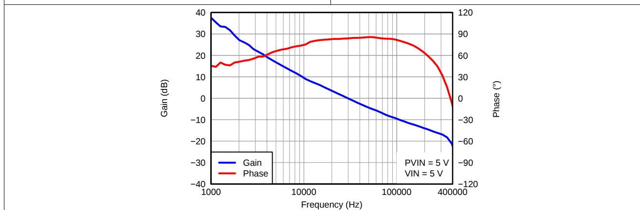
图 10. V OUT =1.2V, I OUT =3A, C OUT1 =47μF 陶瓷电容器, C OUT2 =330μF POSCAP, f SW =480kHz
