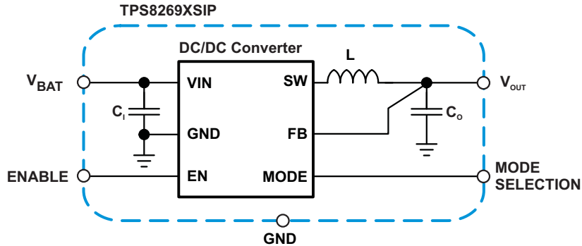
Figure 27. Circuit
