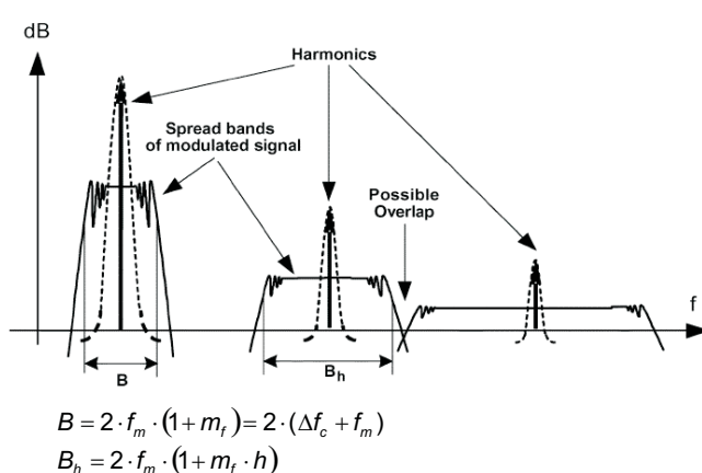
Figure 42. 经调制方波信号中谐波的扩展频带 (1)
