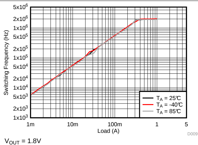
图 22. Switching Frequency
