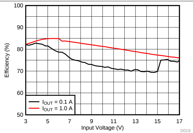
图 7. Efficiency, V_{OUT} = 1.0\text{ V}
