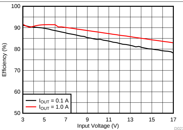
图 9. Efficiency, V_{OUT} = 1.8\text{ V}
