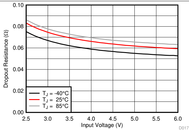
图 1. Dropout Resistance
