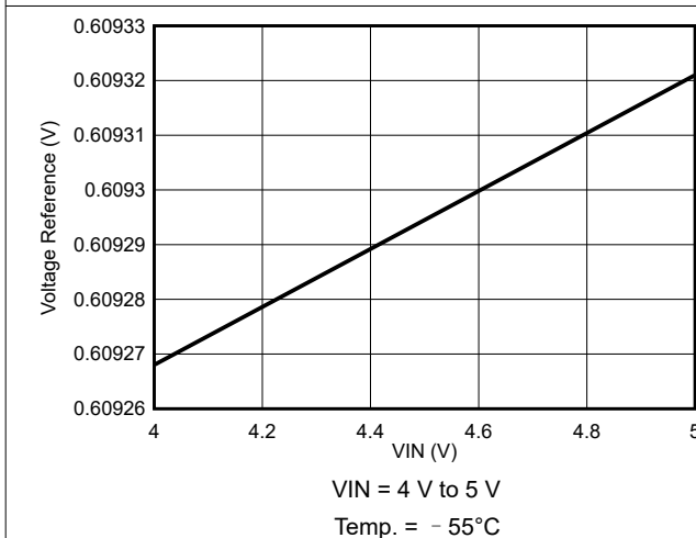
图 7-11. Voltage Reference Variation
