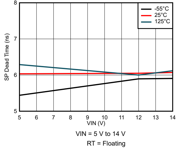
图 7-50. SP Dead Time Variation
