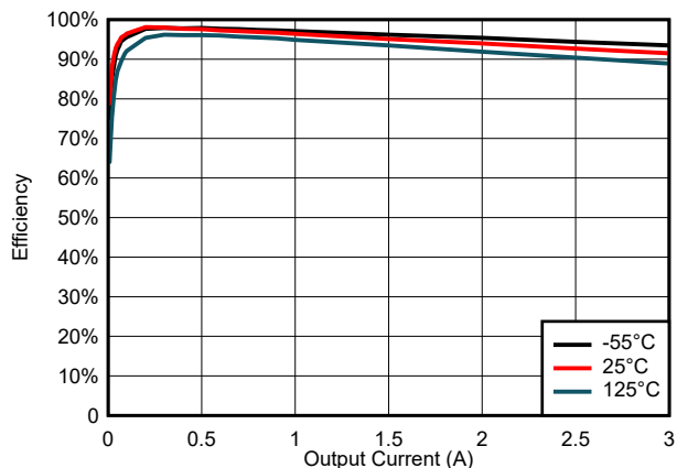
图 6-18. Efficiency for V_{\text{IN}} = 3 \text{ V}
