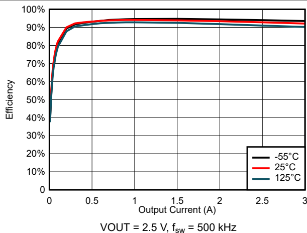
图 6-39. Efficiency for V_{\text{IN}} = 5 \text{ V}
