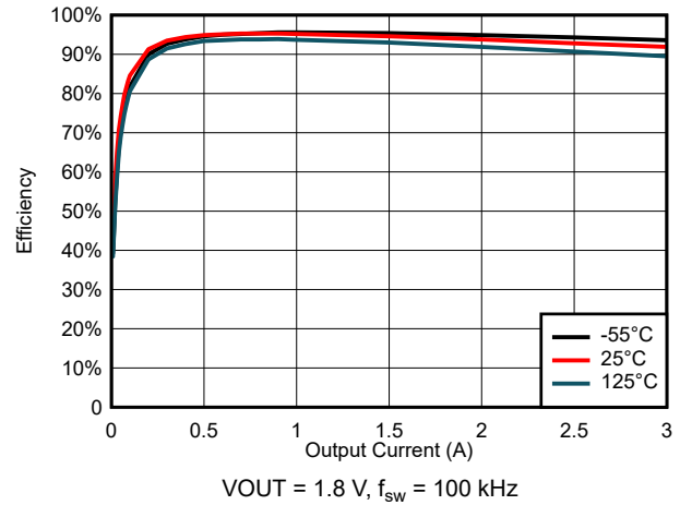
图 6-48. Efficiency for VIN = 5.5 V
