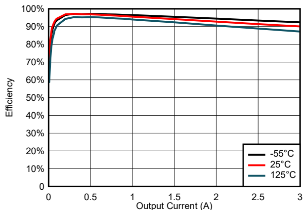
图 6-17. Efficiency for V_{\text{IN}} = 3 \text{ V}
