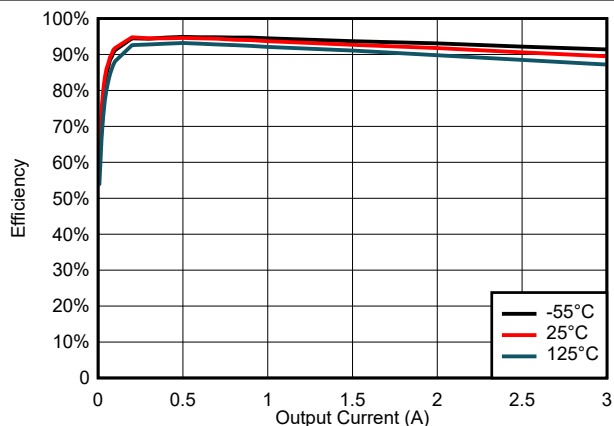
图 6-20. Efficiency for V_{\text{IN}} = 3 \text{ V}
