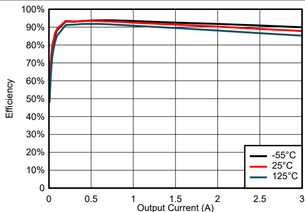
图 6-19. Efficiency for V_{\text{IN}} = 3 \text{ V}
