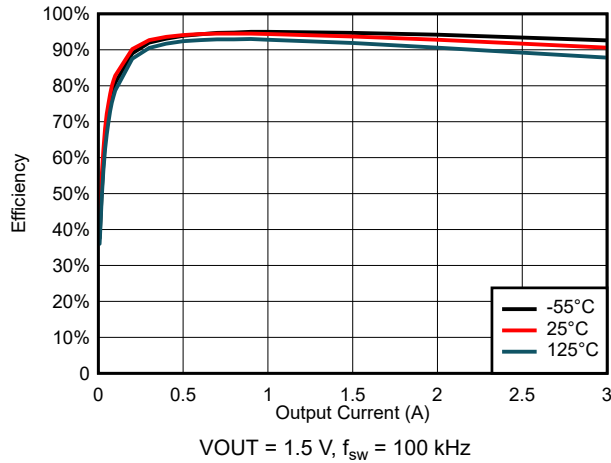
图 6-47. Efficiency for VIN = 5.5 V
