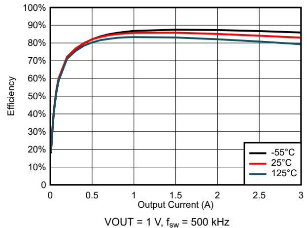
图 6-50. Efficiency for VIN = 5.5 V
