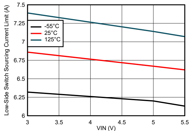
图 6-12. Low-Side Switch Sourcing Current Limit Variation
