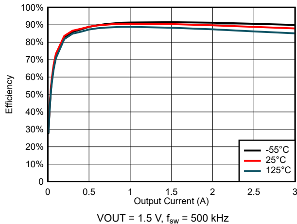
图 6-37. Efficiency for V_{\text{IN}} = 5 \text{ V}
