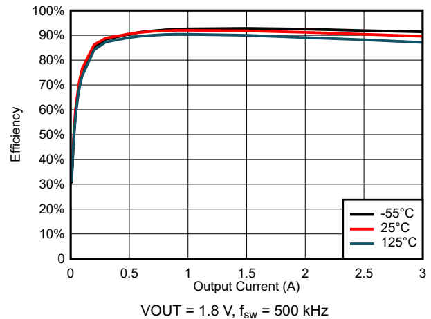
图 6-38. Efficiency for V_{\text{IN}} = 5 \text{ V}
