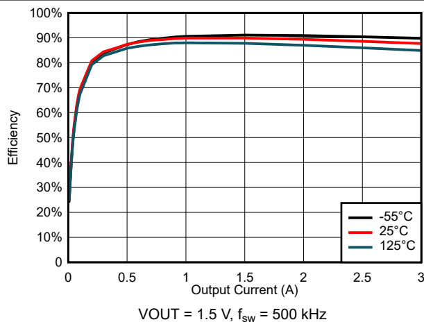
图 6-51. Efficiency for VIN = 5.5 V
