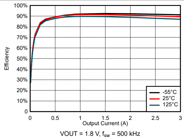
图 6-52. Efficiency for VIN = 5.5 V
