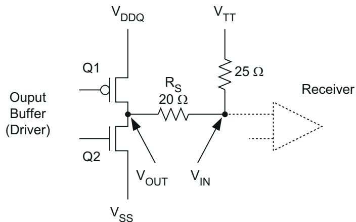
图 8-6. DDR Physical Signal System SSTL Signaling
