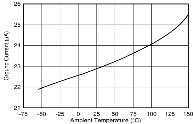
图 6-31. Ground Current at 500 \mu\text{A}
