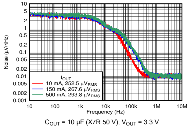
图 6-13. Noise vs Frequency
