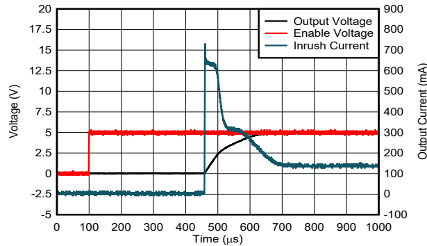
图 8-8. Power-Up Waveform With EN
