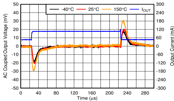
图 6-19. Load Transient, 45 mA to 105 mA
