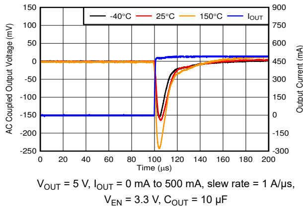
图 6-25. Load Transient, No Load to 500-mA Rising Edge
