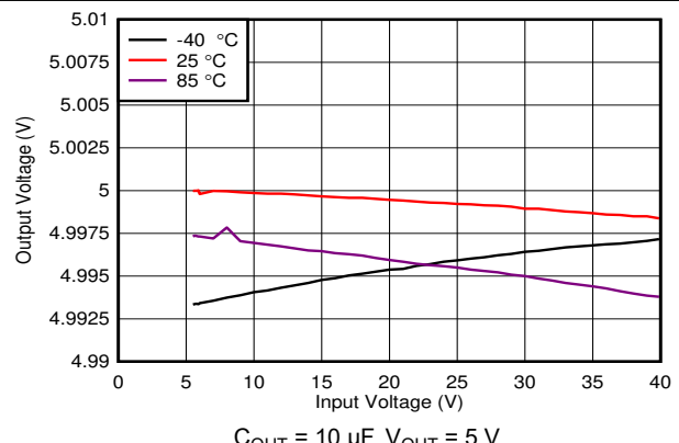
图 6-6. Line Regulation at 50 mA
