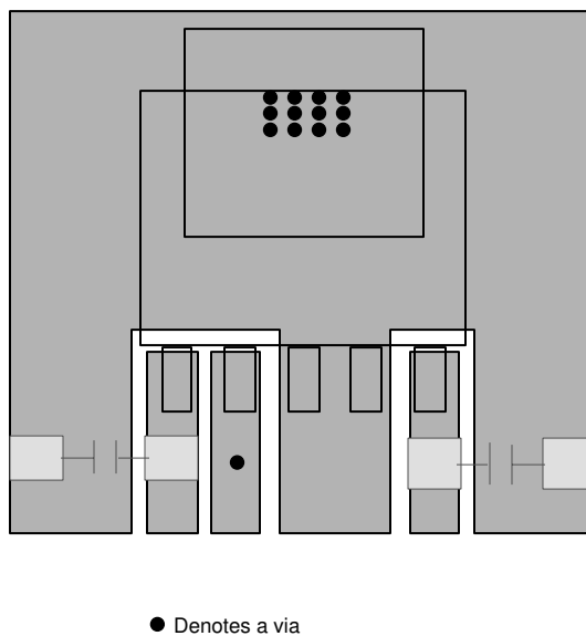
图 8-12. KVV Package Fixed Outupt
