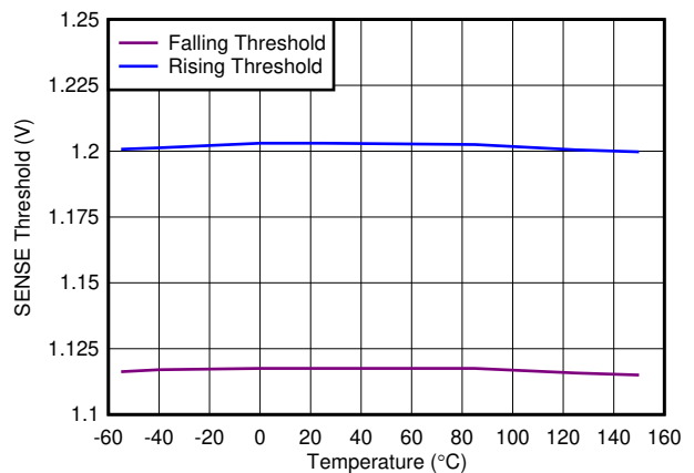
图 6-28. Undervoltage Lockout (UVLO) Threshold vs Temperature
