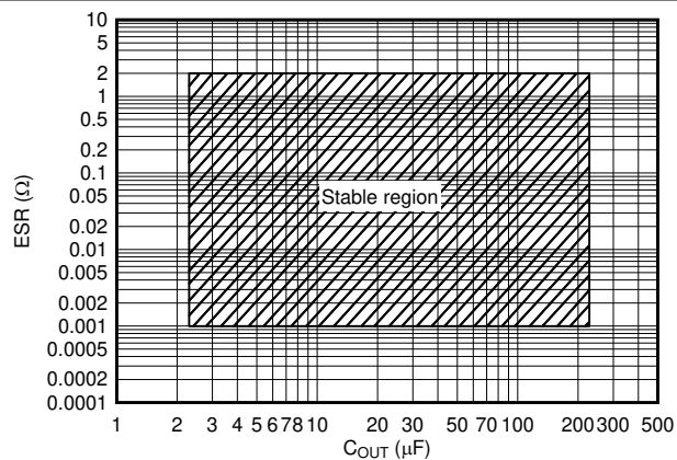
图 6-38. Stability ESR vs C_{OUT}
