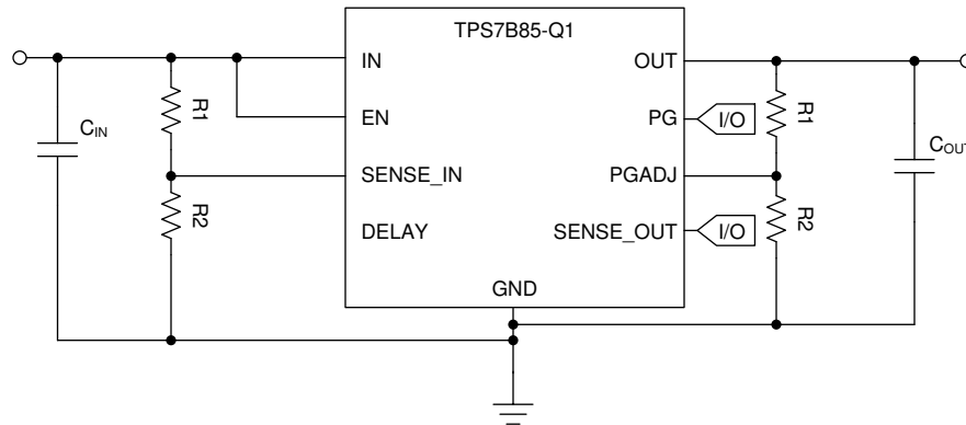
图 8-12. Typical Application Schematic for the TPS7B85-Q1
